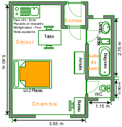
Type A ± 23.50 m 2
